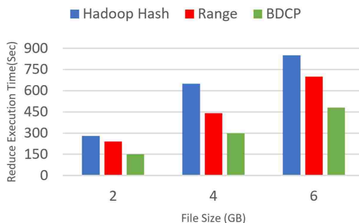
Figure 6.15: Word count job on files of sizes, 2, 4, and 6 GB. Skew degree is 1.1.in heterogeneous cluster
